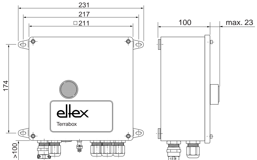
Fig. 14: Dimensions Terra- box TCB030
